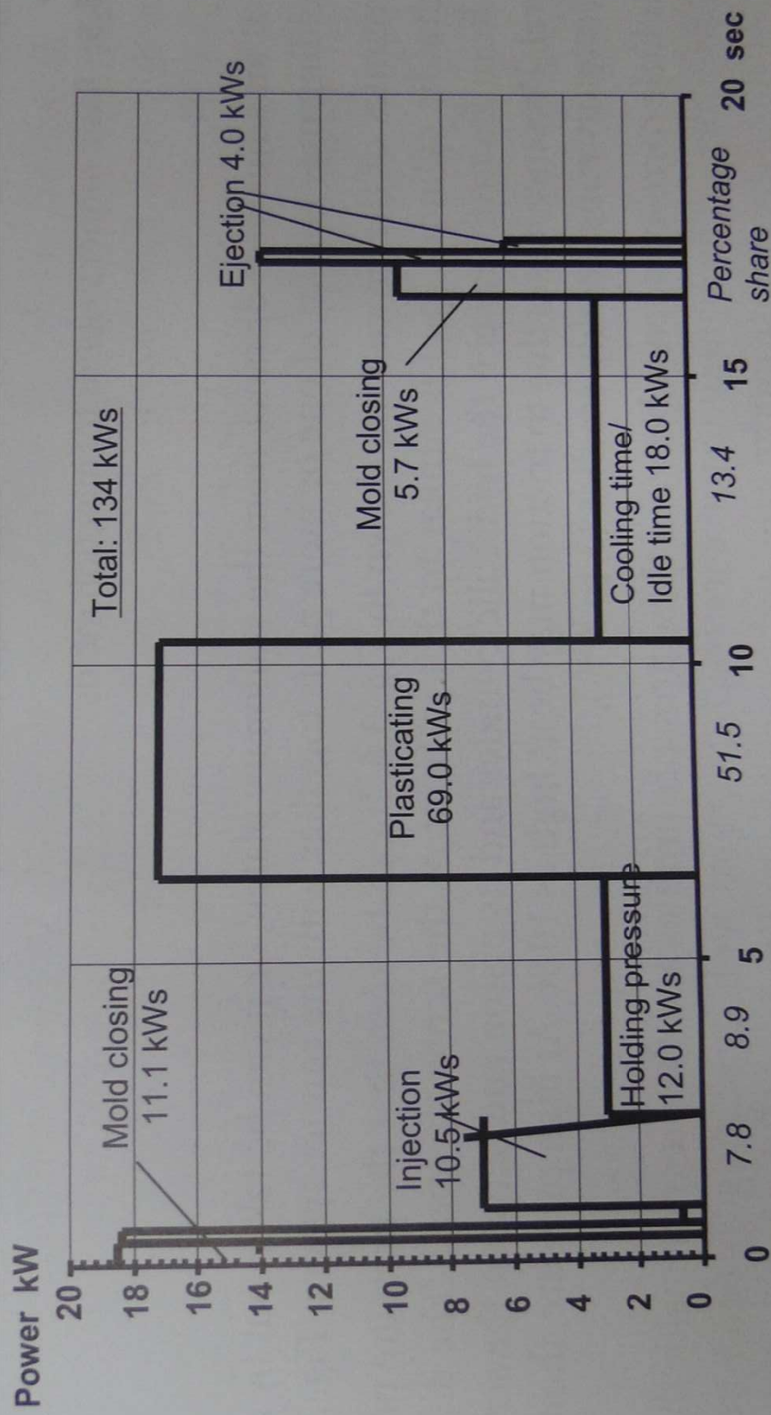
Figure 3.4: The stages of injection molding showing the energy consumption during the different processing steps
