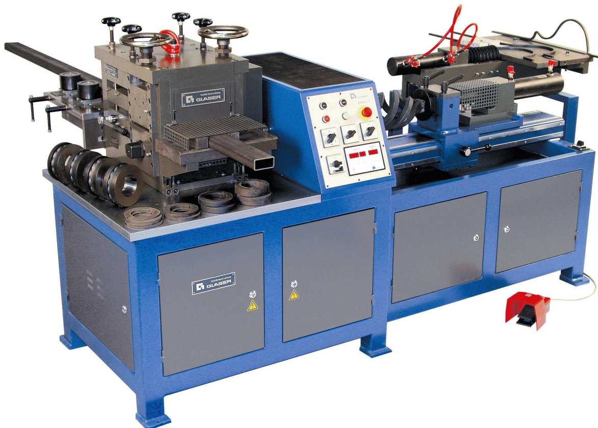
Automatic Multiple-Purpose Iron Twister GDM 50-3 with 27 tons Hydraulic-Device, Pressing Bed and additional Profile-Rolling Device GPG 999
